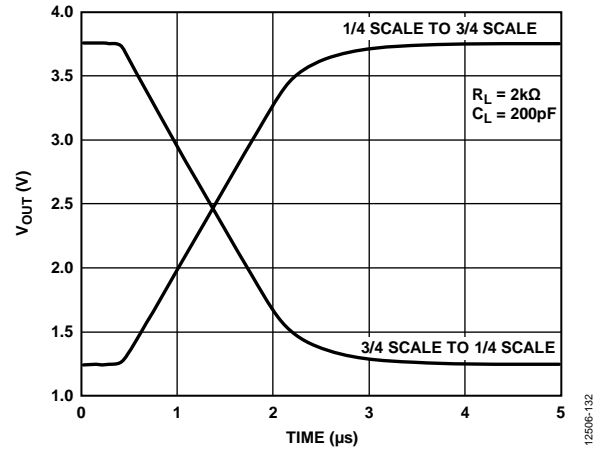
Figure 22. DAC Settling Time, Output Range = 0 V to 2 × VREF
