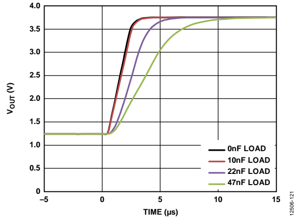
Figure 23. DAC Settling Time for Various Capacitive Loads
