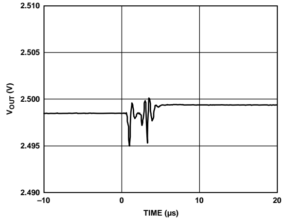
Figure 17. DAC Digital-to-Analog Glitch (Rising)
