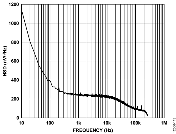
Figure 32. Reference Noise Spectral Density (NSD)
