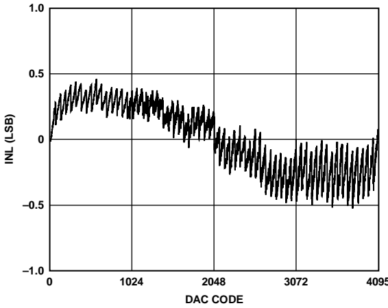
Figure 14. DAC INL
