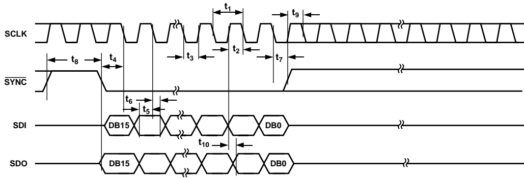
Figure 4. Timing Diagram
