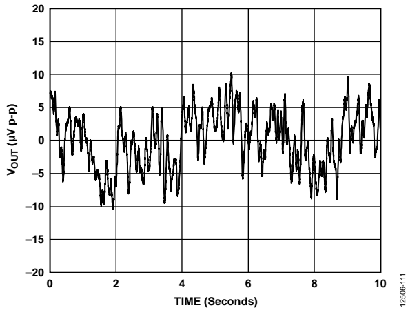
Figure 31. Internal Reference 1/f Noise
