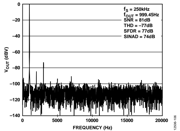
Figure 24. DAC Sine Wave Output, Output Range = 0 V to 2 × VREF, Bandwidth = 0 Hz to 20 kHz
