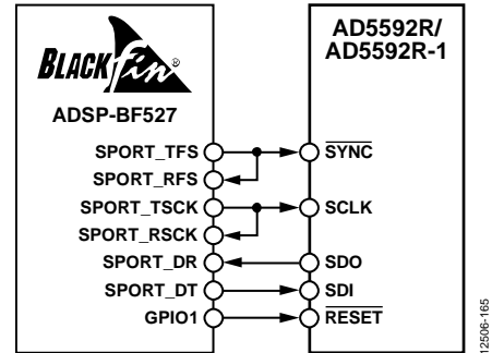
Figure 45. ADSP-BF527 SPORT Interface
