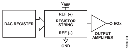
Figure 34. Internal Block Diagram of the DAC Architecture
