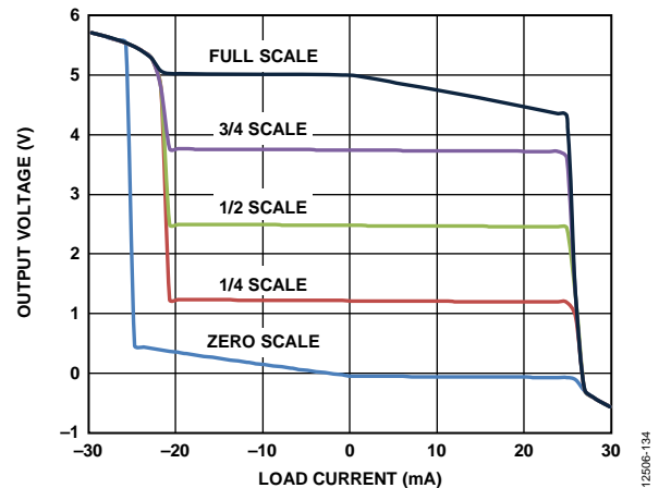
Figure 30. DAC Output Sink and Source Capability, Output Range = 0 V to 2 \times V_{REF}
