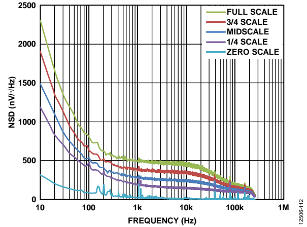
Figure 28. DAC Output Noise Spectral Density (NSD)
