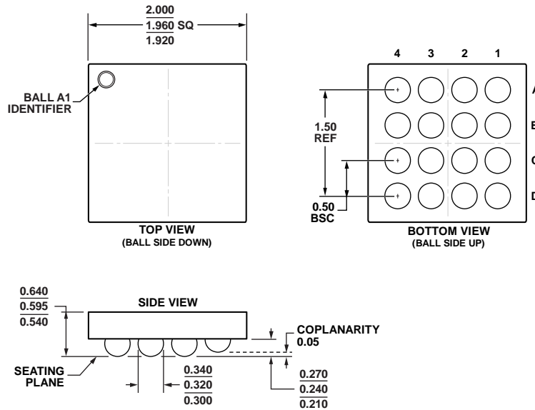
Figure 47. 16-Ball Wafer Level Chip Scale Package [WLCSP] (CB-16-3) Dimensions shown in millimeters
