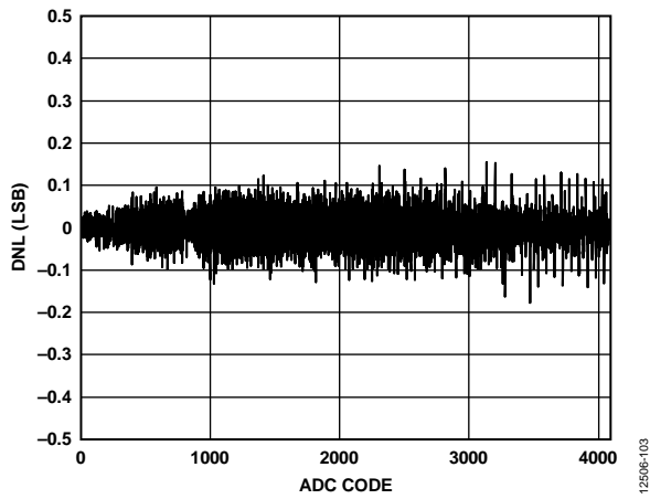
Figure 8. ADC DNL, V_{DD} = 5.5V
