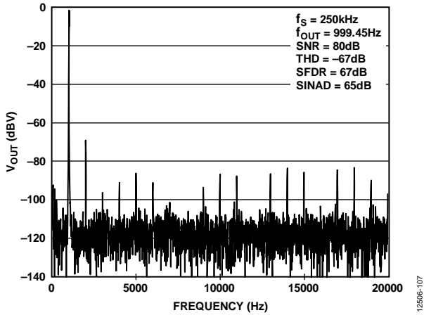
Figure 25. DAC Sine Wave Output, Output Range = 0 V to V_{REF} , Bandwidth = 0 Hz to 20 kHz
