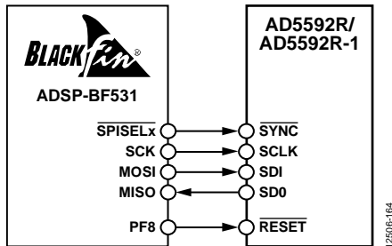
Figure 44. ADSP-BF531 SPI Interface
