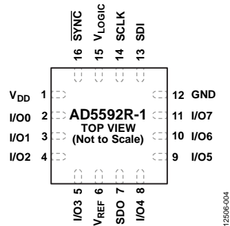
Figure 6. AD5592R-1 16-Lead LFCSP Pin Configuration
