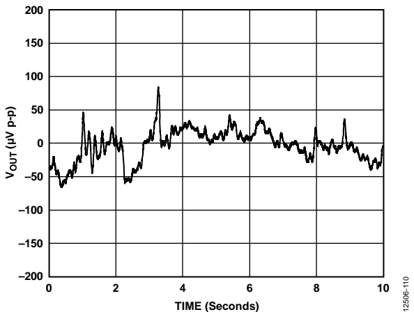
Figure 27. DAC 1/f Noise with Internal Reference
