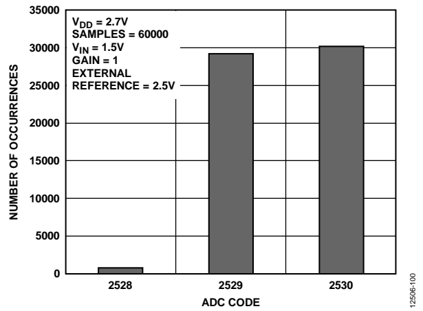
Figure 11. Histogram of ADC Codes, V_{DD} = 2.7V
