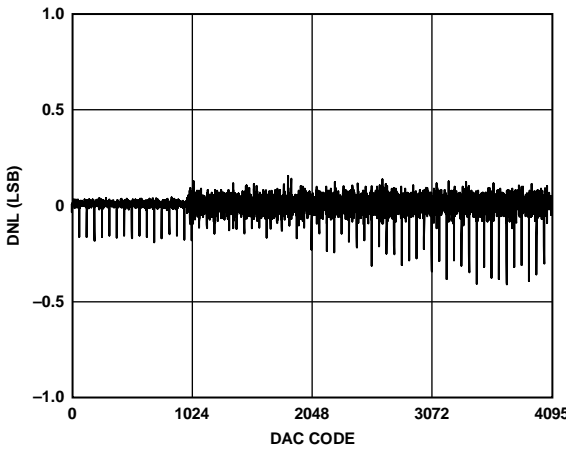
Figure 15. DAC DNL
