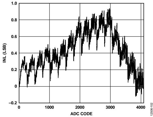
Figure 7. ADC INL, V_{DD} = 5.5V
