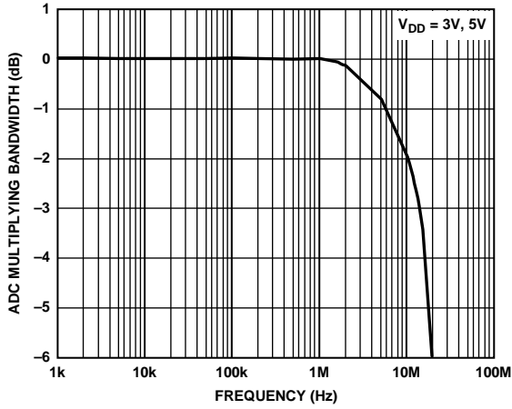
Figure 13. ADC Multiplying Bandwidth
