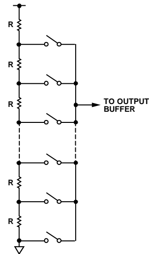
Figure 35. Simplified Resistor String Structure
