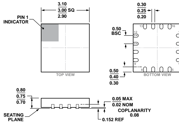
Figure 46. 16-Lead Lead Frame Chip Scale Package [LFCSP_WQ] 3 mm x 3 mm Body, Very Very Thin Quad (CP-16-32) Dimensions shown in millimeters
