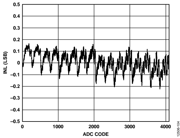
Figure 9. ADC INL, V_{DD} = 2.7V
