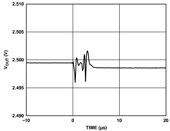
Figure 18. DAC Digital-to-Analog Glitch (Falling)
