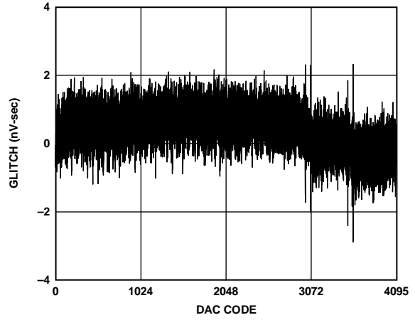
Figure 16. DAC Adjacent Code Glitch
