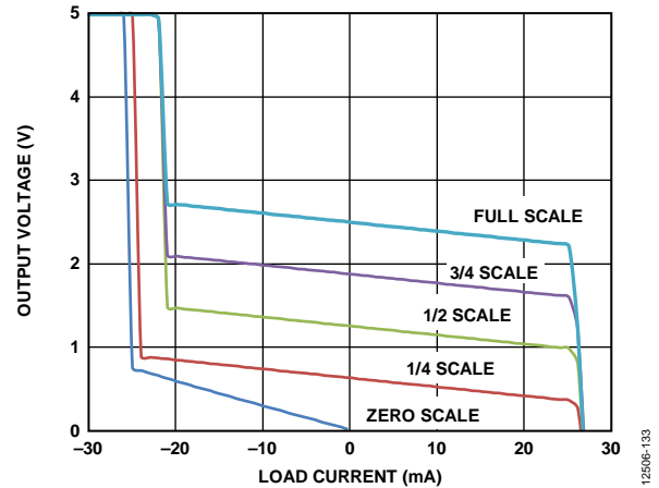
Figure 29. DAC Output Sink and Source Capability, Output Range = 0 V to V_{REF}
