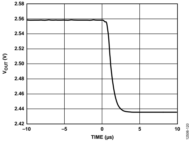
Figure 20. DAC Settling Time (100 Code Change, Falling Edge)
