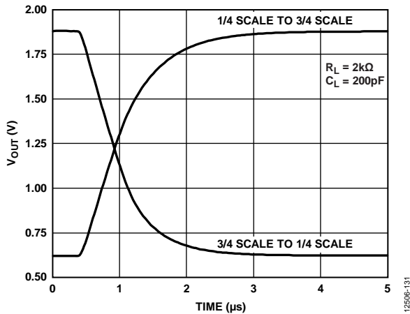
Figure 21. DAC Settling Time, Output Range = 0 V to VREF
