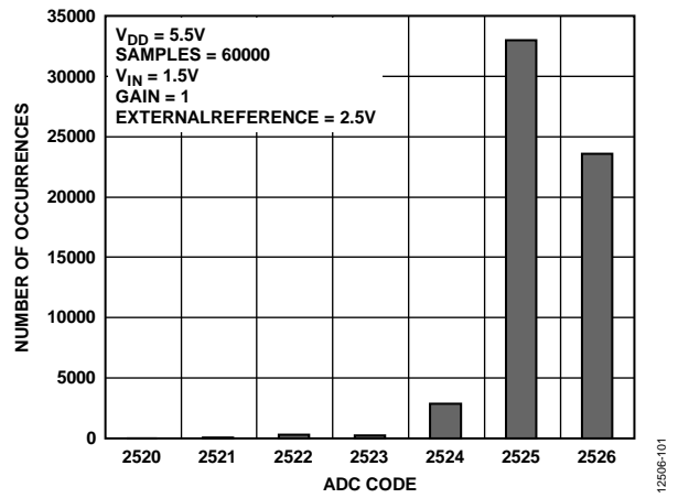
Figure 12. Histogram of ADC Codes, V_{DD} = 5.5V
