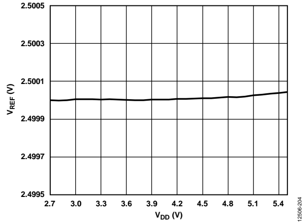
Figure 33. Reference Line Regulation
