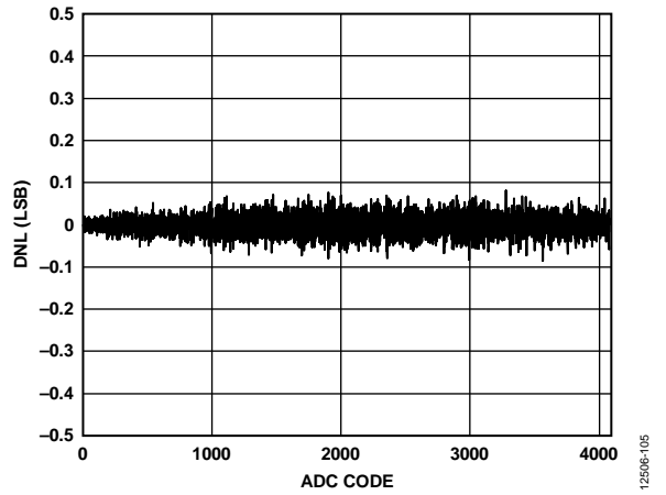
Figure 10. ADC DNL, V_{DD} = 2.7V
