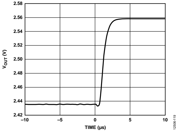
Figure 19. DAC Settling Time (100 Code Change, Rising Edge)
