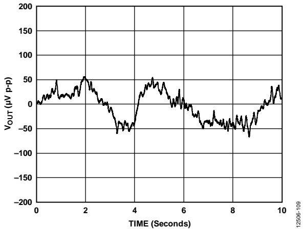
Figure 26. DAC 1/f Noise with External Reference
